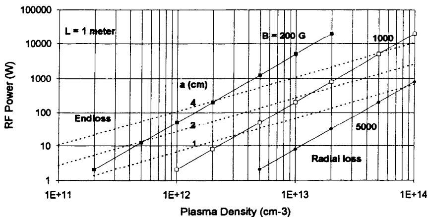
Figure 34. Rf power required to sustain a 1-m long discharge against radial losses ( solid lines ) and axial losses ( dashed lines ), computed separately, vs. plasma density, for various values of tube radius and magnetic field. [34]
