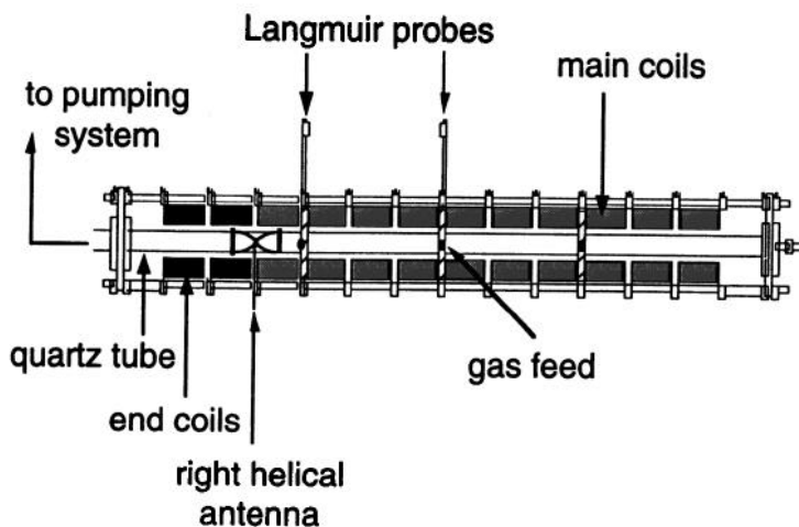
Figure 18. Typical Type A helicon discharge configuration. [85]
