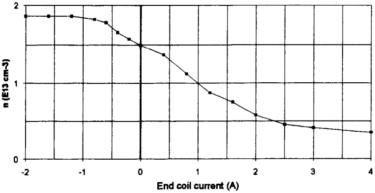
Figure 39. Increase in density on axis with decrease in end-coil current. [34] The current at the extreme right gives a uniform field.
