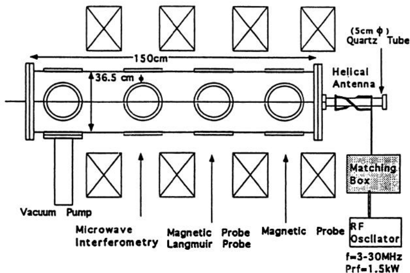
Figure 19. Typical Type B helicon discharge configuration. [82]
