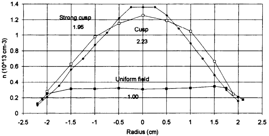
Figure 40. Radial density profiles in the uniform-field region of Fig. 36 for positive, zero, and negative end-coil currents corresponding to the right, center, and left regions of Fig. 37. [37] The numbers on the curves are proportional to the integrated density in each cross section.
