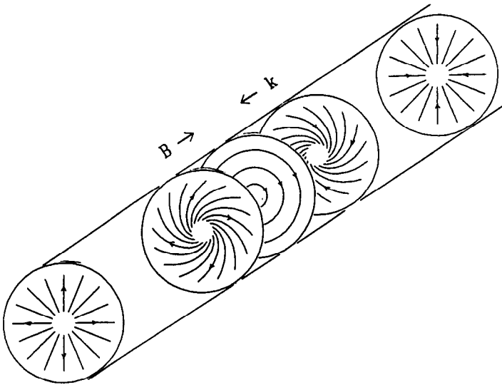
Figure 4. Instantaneous electric field pattern for an m = 0 helicon wave in space. [27]
