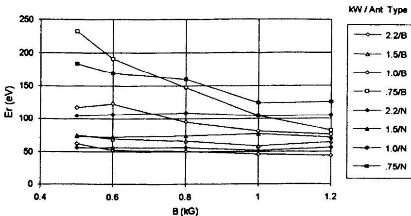
Figure 25. Values of resonant energy E_r , deduced from the slope of the n - B curves. [34] Data taken in a 4-cm diameter tube at 27.12 MHz. The curves refer to different values of RF power and different antennas, B for Boswell-type, and N for Nagoya Type III.
