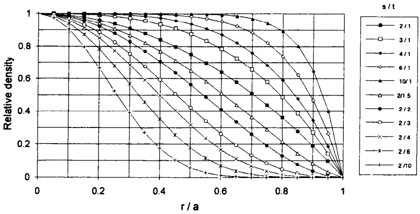
Figure 13. Model density profiles characterized by the parameters s and t . [35]
