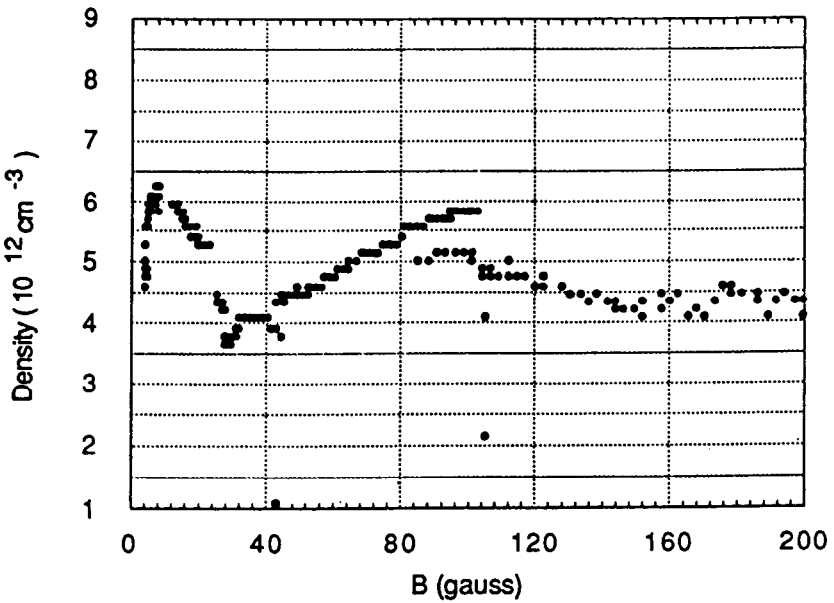
Figure 6. Density peak in a helicon discharge at low magnetic fields, from Ref. 32.
