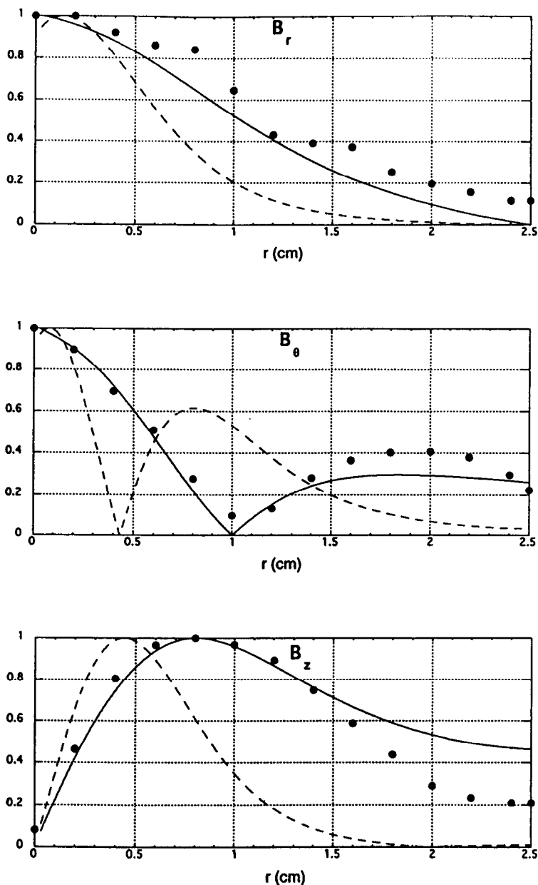
Figure 28. Measurements of the normalized magnitudes of B_r , B_\theta , and B_z for R-wave excitation (Fig. 10) in a 5-cm diameter discharge at 800 G with 1.9 kW of RF at 27.12 MHz. [66] The theoretical curves for the m = +1 (solid) and m = -1 (dashed) modes were computed from the measured density profiles.
