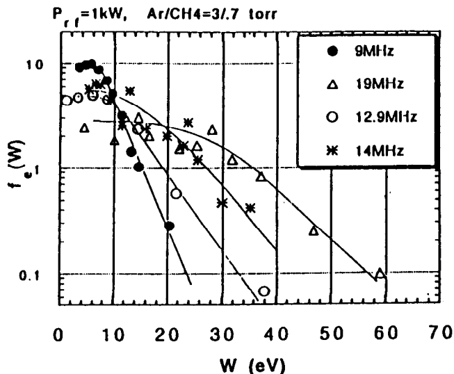
Figure 32. Electron energy distribution f(W) in an \text{Ar}/\text{CH}_4 helicon discharge at various RF frequencies. [80]
