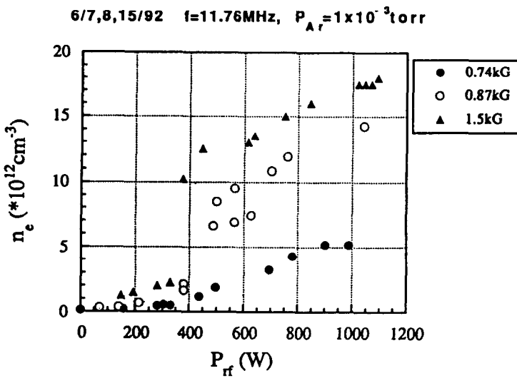
Figure 22. Discontinuous jump in density with increase in RF power. [82]
