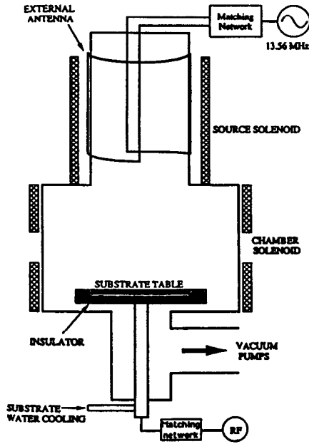
Figure 20. Typical Type C helicon discharge configuration. [74]
