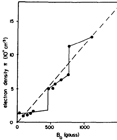
Figure 21. Stepwise linear n - B relation observed at low power (180 W) and 1 kG. [10]
