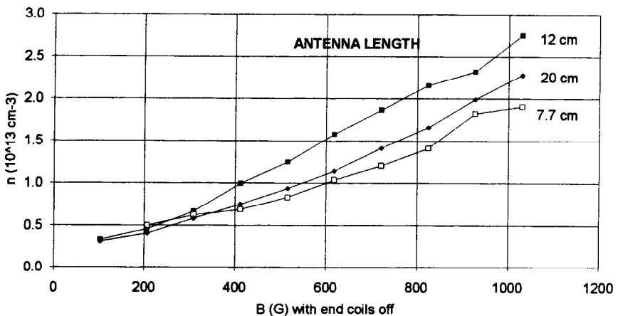
Figure 36. Peak density vs. magnetic field for Nagoya Type III antennas of different lengths. [34] Parameters were: a = 2 cm, p = 4 mtorr of argon, P_{rf} = 2.2 kW at 27.12 MHz.
