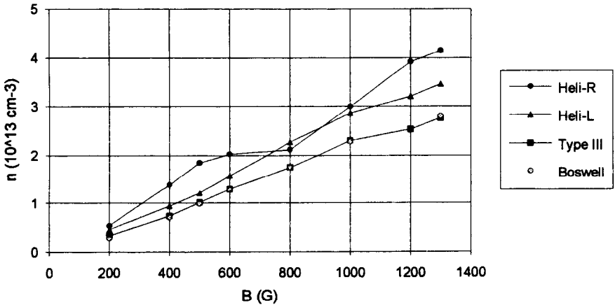
Figure 37. Peak density vs. magnetic field for four 12-cm long antennas of different designs. [34] Parameters were as in Fig. 36.
