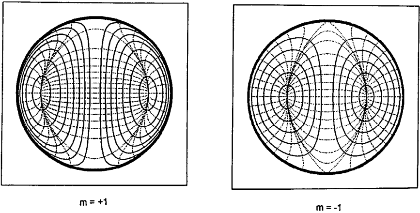
Figure 2. Pattern of magnetic ( solid ) and electric ( dashed ) field lines in the m = +1 and -1 modes of the helicon wave in a uniform plasma in a plane perpendicular to the DC magnetic field. [35]
