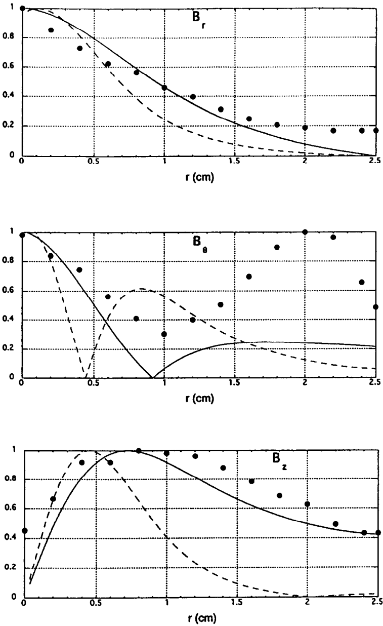
Figure 29. Same as Fig. 28 but for L -wave excitation (Fig. 11).
