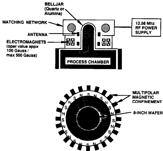
Figure 43. Schematic of the MORI etching tool of PMT, Inc., employing a 10-cm diameter helicon source. The process chamber is 36 cm in diameter, accommodating 20-cm diameter wafers in a cooled chuck, located about 20 cm below the source. [18]
