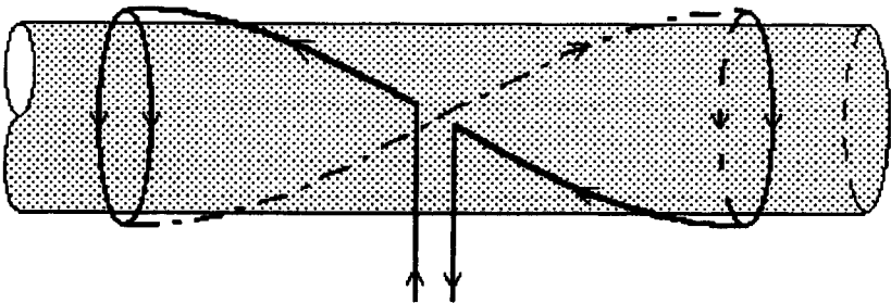
Figure 11. Schematic of a left-hand helical antenna.
